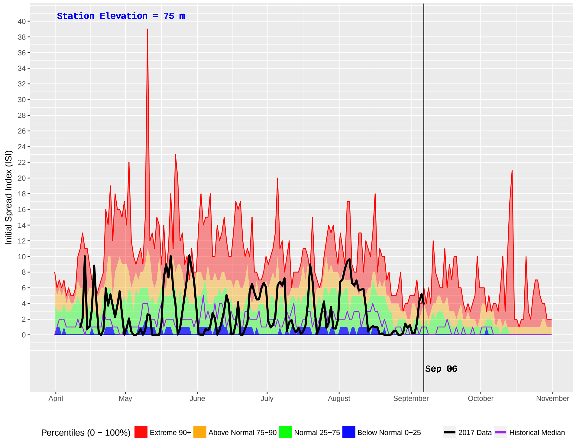
KITPARK (106) : Historical (1995–2016) and Current (2017) Noon Initial Spread Index (ISI)
