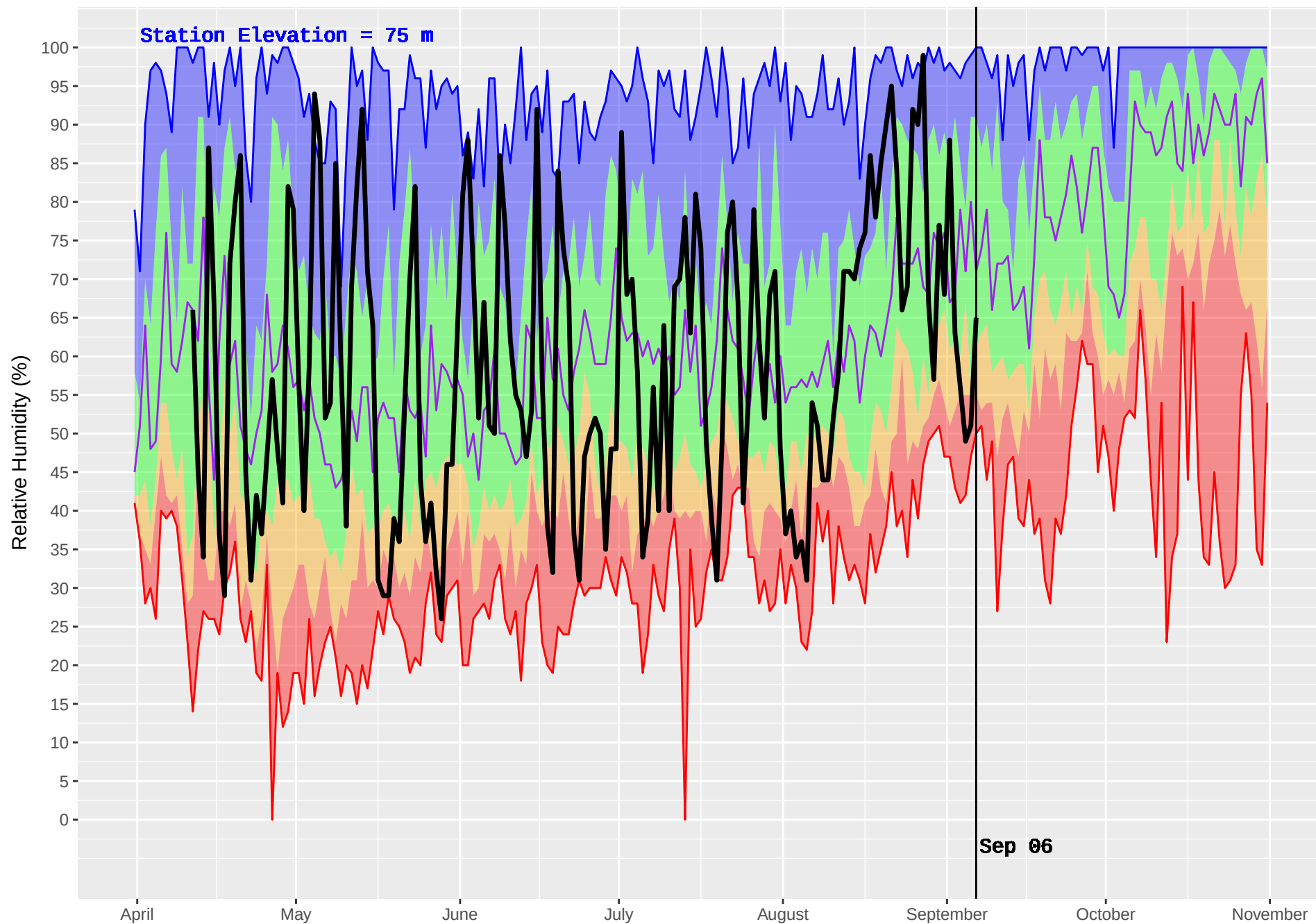
KITPARK (106) : Historical (1995–2016) and Current (2017) Noon Relative Humidity
