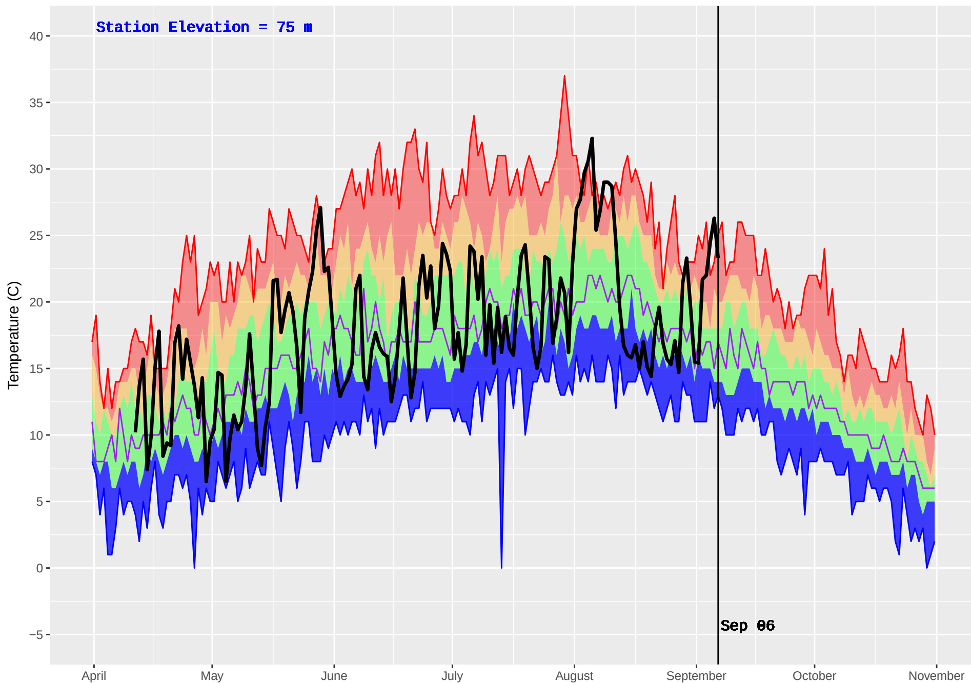
KITPARK (106) : Historical (1995–2016) and Current (2017) Noon Temperature
