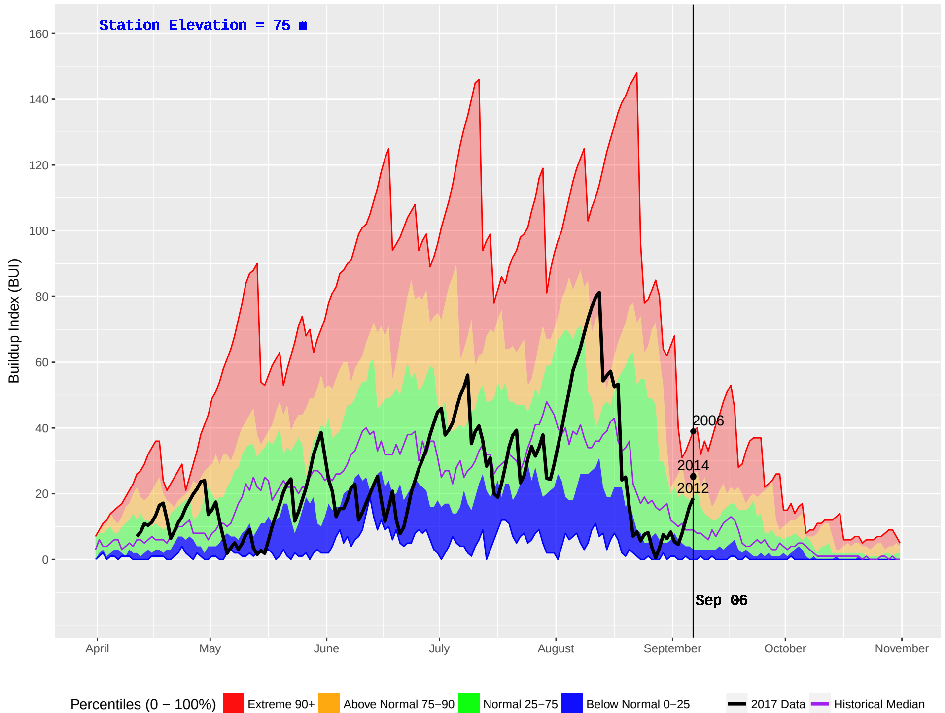
KITPARK (106) : Historical (1995–2016) and Current (2017) Noon Buildup Index (BUI)
